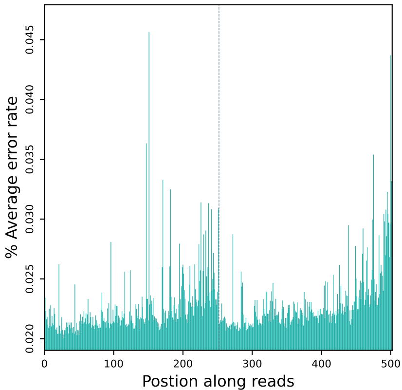
Error rate distribution along reads (R20112)
